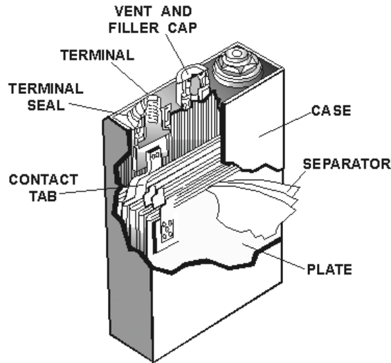
Figure 2-11.—Nickel-cadmium cell.
